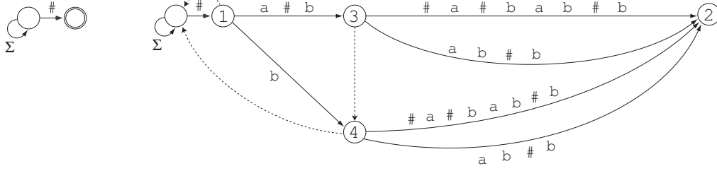
Figure 2. To the left is the minimum DFA M_D accepting dictionary D = \Sigma^*\# . To the right is SCDAWG_D(u) with u = \mathbf{a\#b\#a\#bab\#b} , where Node 1 is its source node. The suffix links are displayed by broken arrows. Nodes 1 and 4 are those of Group 1, Node 3 is that of Group 2, and Node 2 is that of Group 3 of Definition 14.
